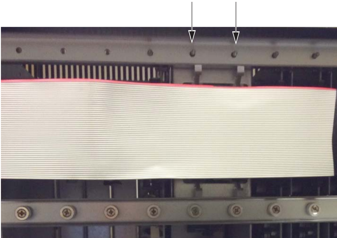
Figure 5. Guide pins and guide holes inside the Stage 64
