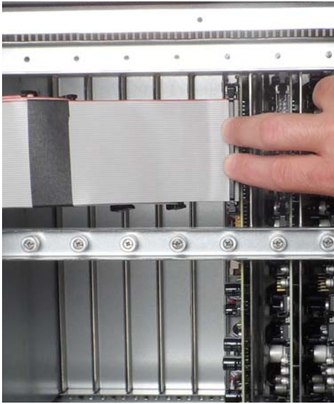
Figure 8. Connecting ribbon cable (your installation may appear differently depending on the slots used for the DNT-192 card)
